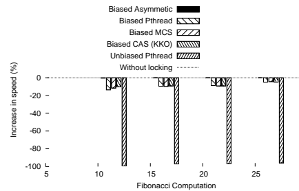
Figure 10: Lock overhead for a sequential program
