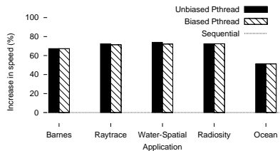
Figure 15: Performance of our biased locks on applications (SPLASH2 benchmark) without dominant behavior.
