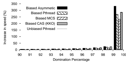
Figure 9: Behavior at high domination percentages
