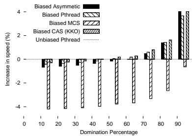
Figure 8: Behavior at varying domination percentages
