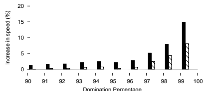
Figure 13: The effect of bias transfer
