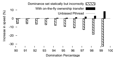
Figure 14: The effect of bias transfer for incorrect biasing
