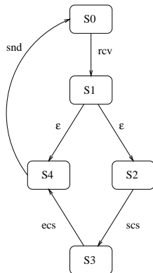
Figure 2: Template process for the Mutual Exclusion Protocol
