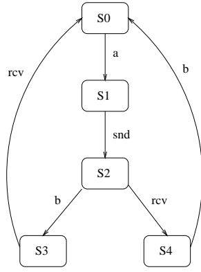
Figure 3: Template process for Milner's Scheduler Protocol
