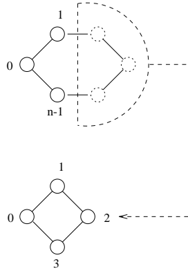
Figure 1: The abstraction used in the proof of Theorem 5
